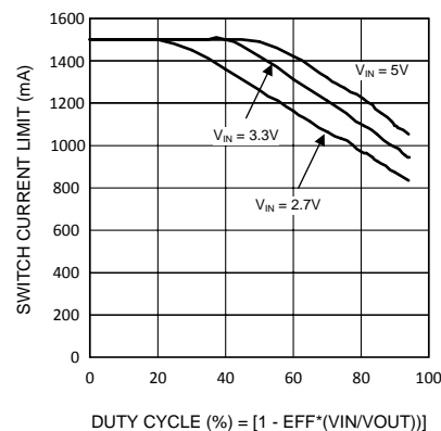
Figure 29. Switch Current Limit vs Duty Cycle - "Y"
