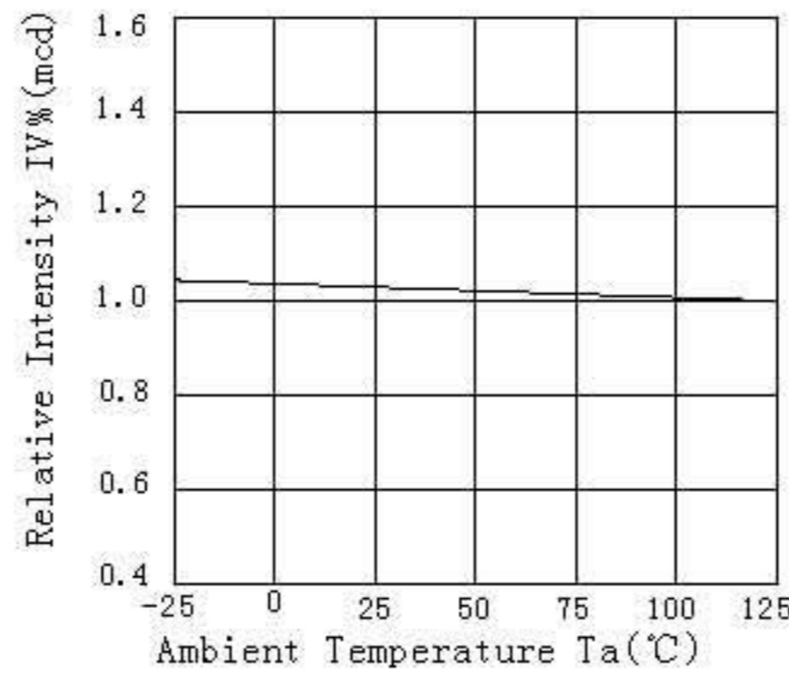
Relative Intensity IV% (mod) vs. Ambient Temperature
