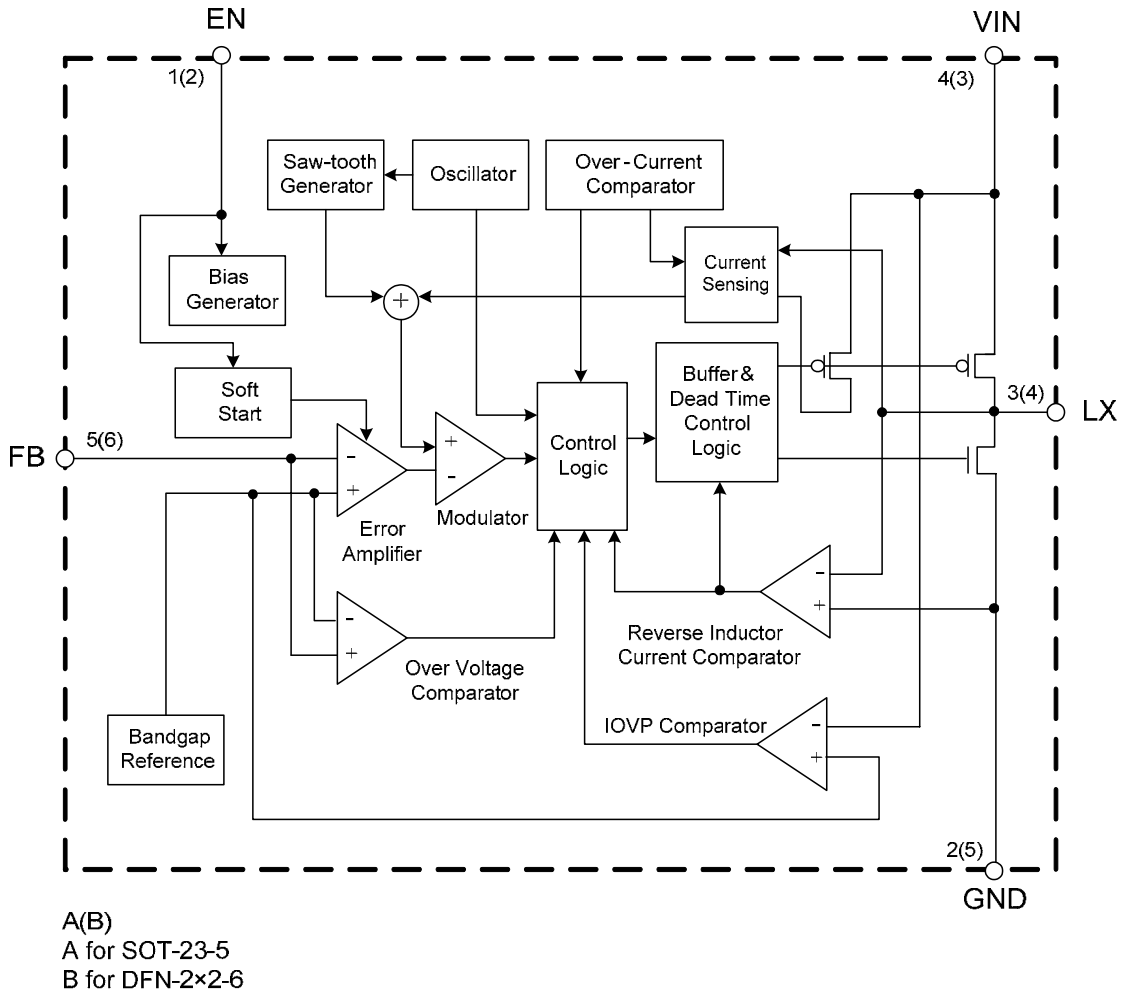
Figure 3. Functional Block Diagram of AP3417C
