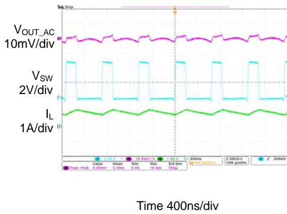
Figure 7. Output Ripple ( I_{OUT}=1A )
