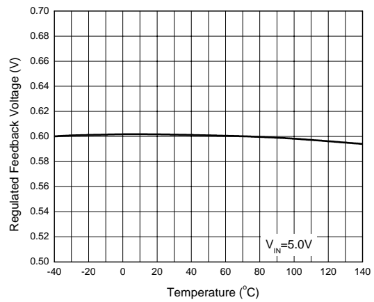
Figure 5. Regulated Feedback Voltage vs. Temperature
